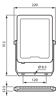
BVP165 LED120/865 PSU 100W SWB CE
